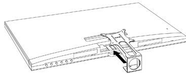
B (x4) M4x12mm Thumbscrew
